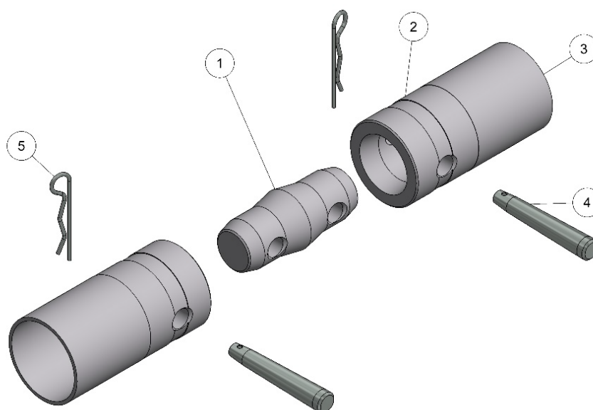
Figure 1: Conical connection
