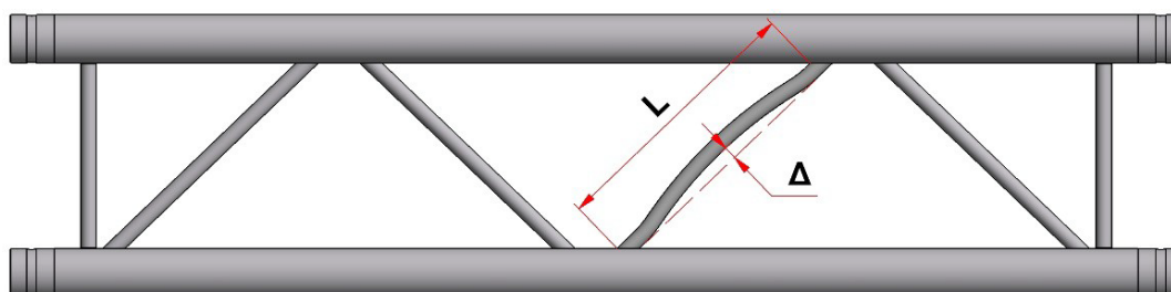
Figure 18: Bent diagonal
