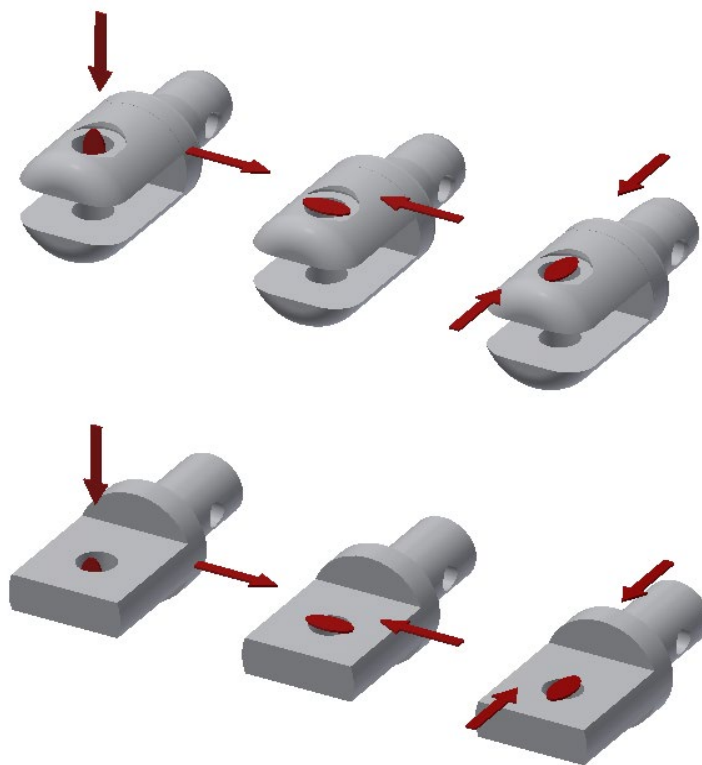
Figure20: pin fork connections
