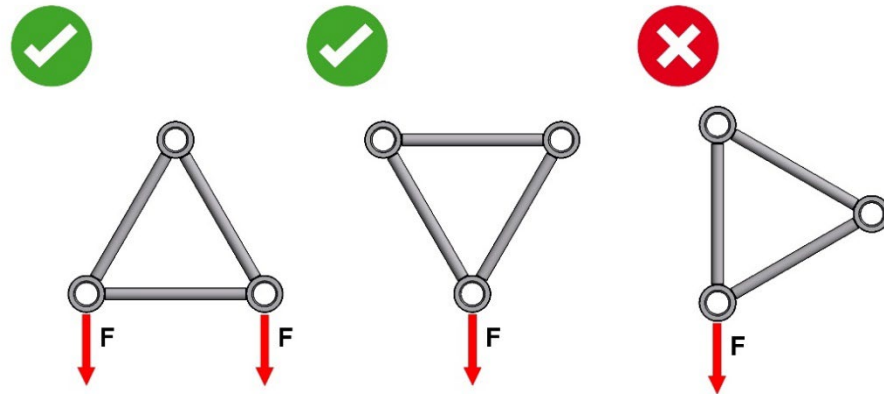
Figure 13: Attaching loads to a triangular truss
