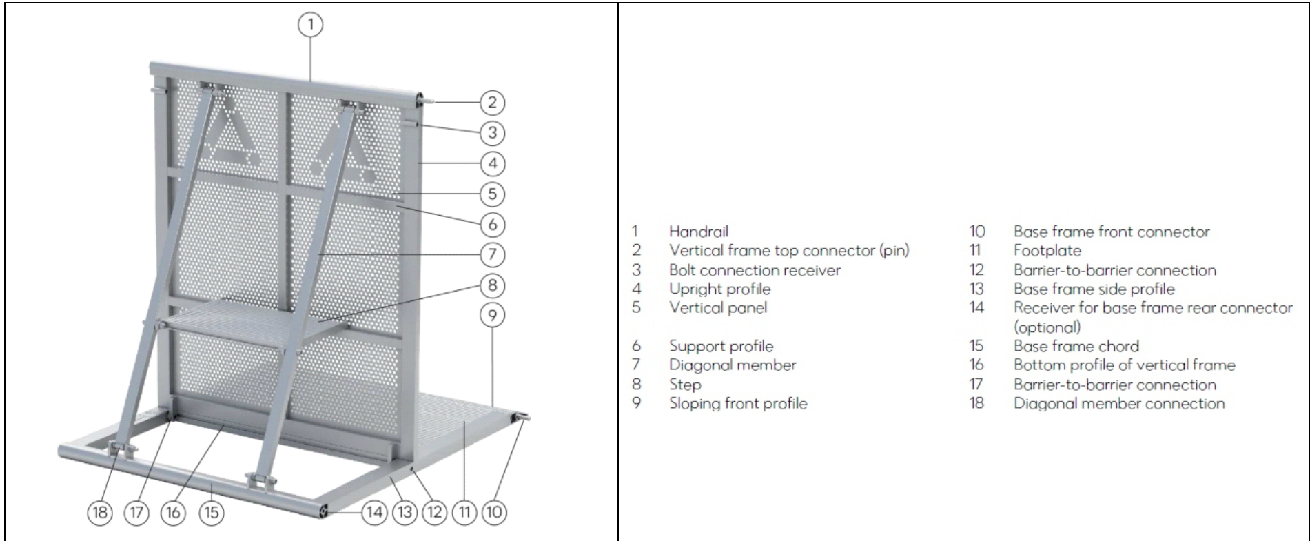
Abb. 1: Wellenbrecher Typ BAR-30-100 Figure 1: Crowd barrier BAR-30-100
